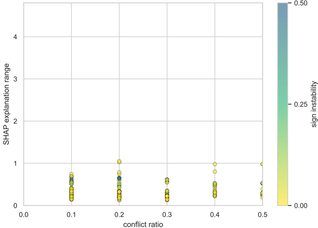
cat__service_http: SHAP explanation range (Spearman r = 0.089 )
